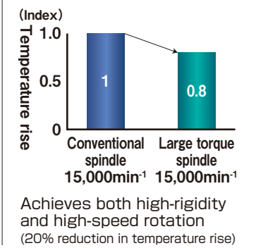
Minimizes heat generation in the high speed ranges (front bearing exhaust temperature)
