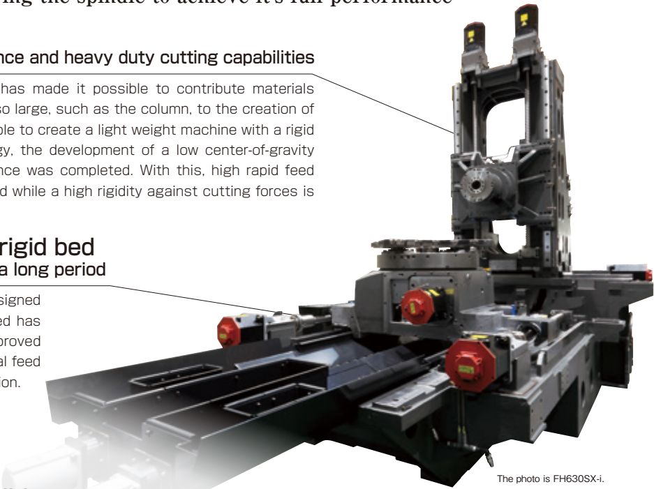
The photo is FH630SX-I.
