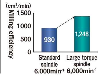
Efficient face milling in low speed ranges
