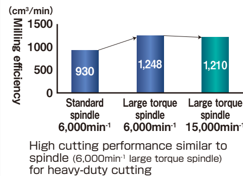
Efficient face milling in low speed ranges
