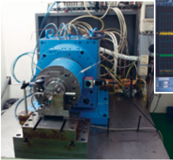
High-speed spindle running rest
