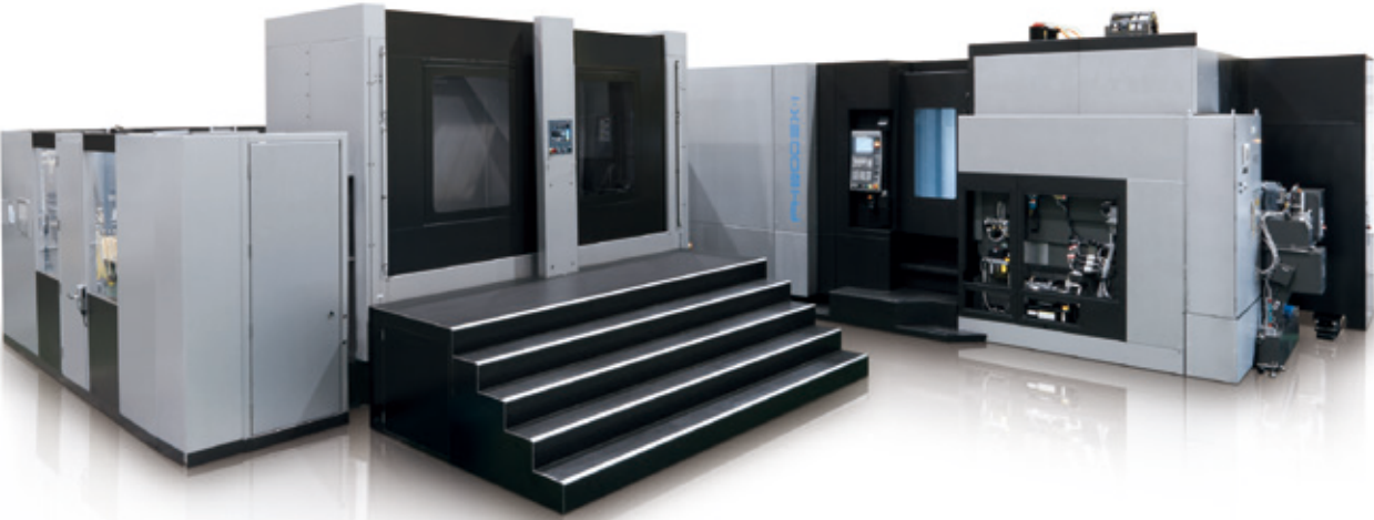
This is an example of FH800SX-I and RGV (rail guided vehicle)
